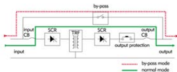
IMPACT 1XX 1 PHASE STATIC VOLTAGE REGULATOR
